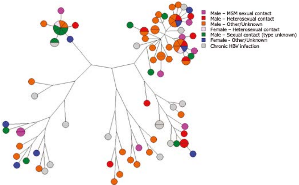
Figure 7.3.3 Optimised maximum parsimony tree based on the full-length sequence of HBV cases in the Netherlands in 2019 by reported transmission route (n=94). gX: genotype
